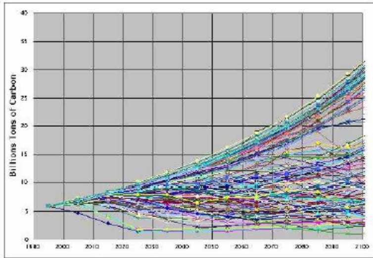
Fig. 1. A Landscape of Plausible Futures showing a wide range of future greenhouse gas emissions paths all consistent with available information.
